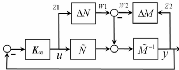
Figure 1. Robust stabilization with respect to the co prime factor uncertainties
