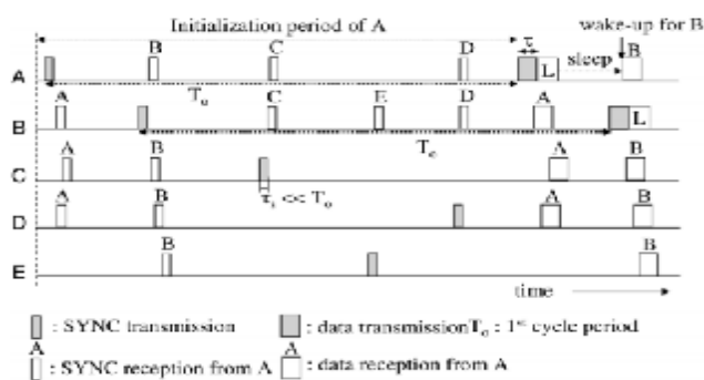
Figure 3. Initialization phase in UWAN-MAC [3]
