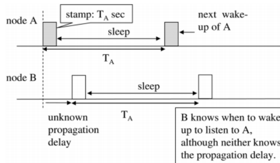
Figure 2. Listen cycle determination in UWAN-MAC [3]
