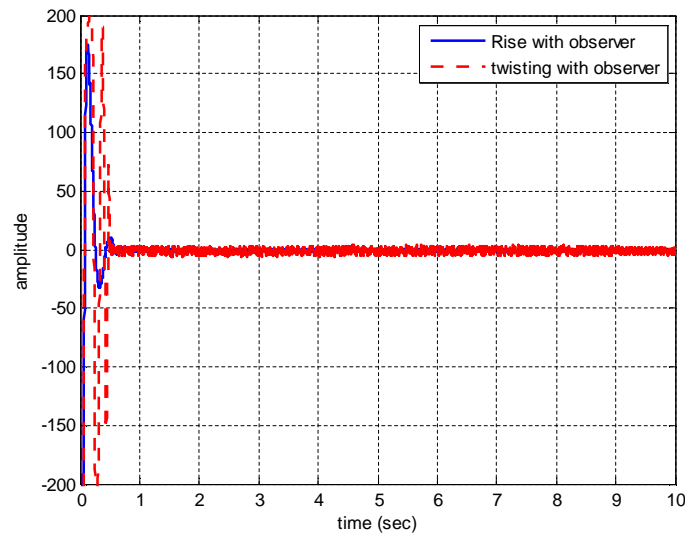
Figure 7. Control effort
