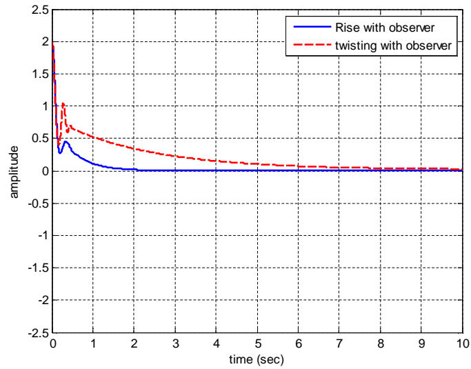
Figure 3. State x_1 applying Rise feedback controller in comparison with twisting algorithm
