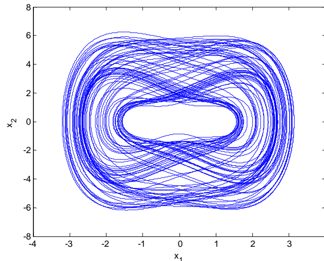
Figure 2. Chaotic behavior of modified Duffing system in 250 seconds
