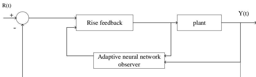
Figure 1. Block diagram of proposed control strategy
