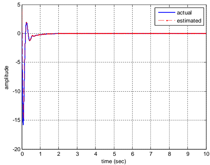
Figure 4. State x_2 applying Rise feedback controller and its estimation
