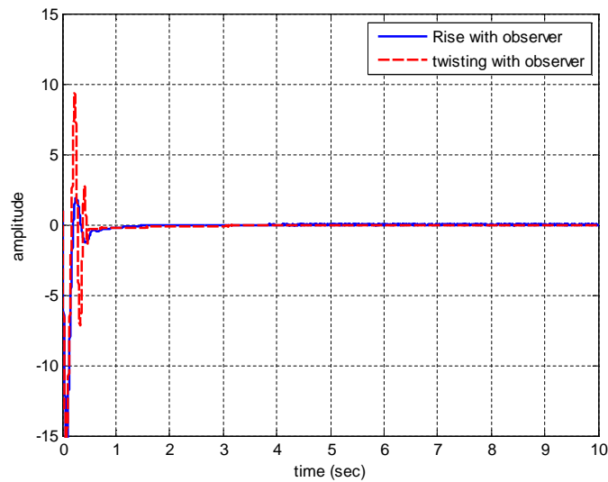
Figure 6. State x_2 applying Rise feedback controller in comparison with twisting algorithm
