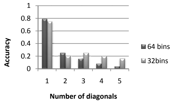
Figure 4. Impact of the number of diagonals. Performance of the matching procedure is fallen dramatically bu increasing the number of diagonals
