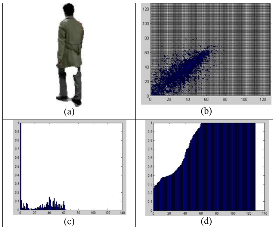
Figure 1. (a) image of a person (b) co-occurrence matrix of Y channel (c) Diagonal vector of b (d) Cumulative distribution of c
