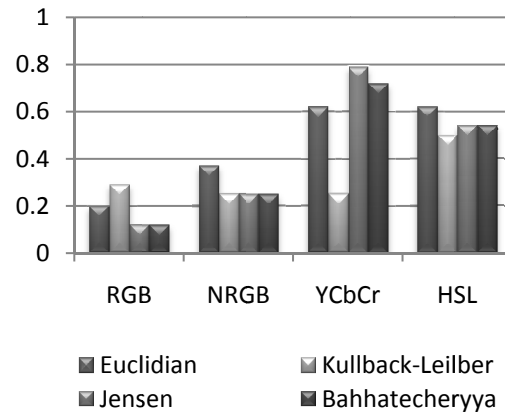
Figure 3. Accuracy of object matching with proposed method in different color spaces
