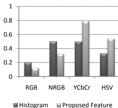
Figure 2. Accuracy of the proposed method comared with color histogram
