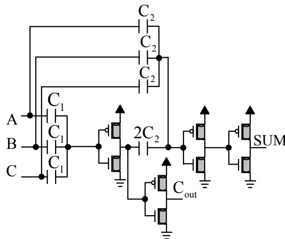
Figure 1. The schematic of Design2 [11]
