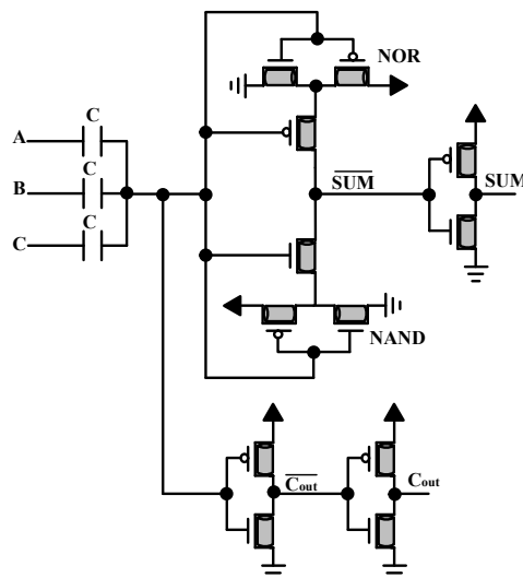
Figure 4. The schematic of FA2 [14]
