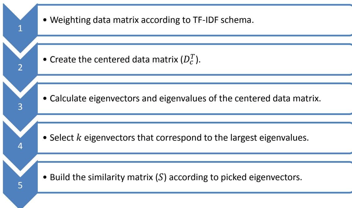
Figure 1: The overall picture of the proposed semantic kernel.
