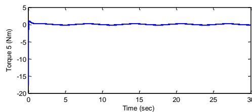
6(l). Control input to joint 5
