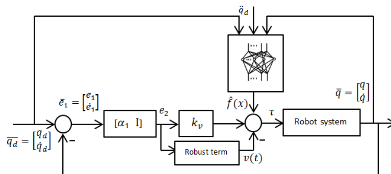
Figure 4. Multilayer NN controller structure
