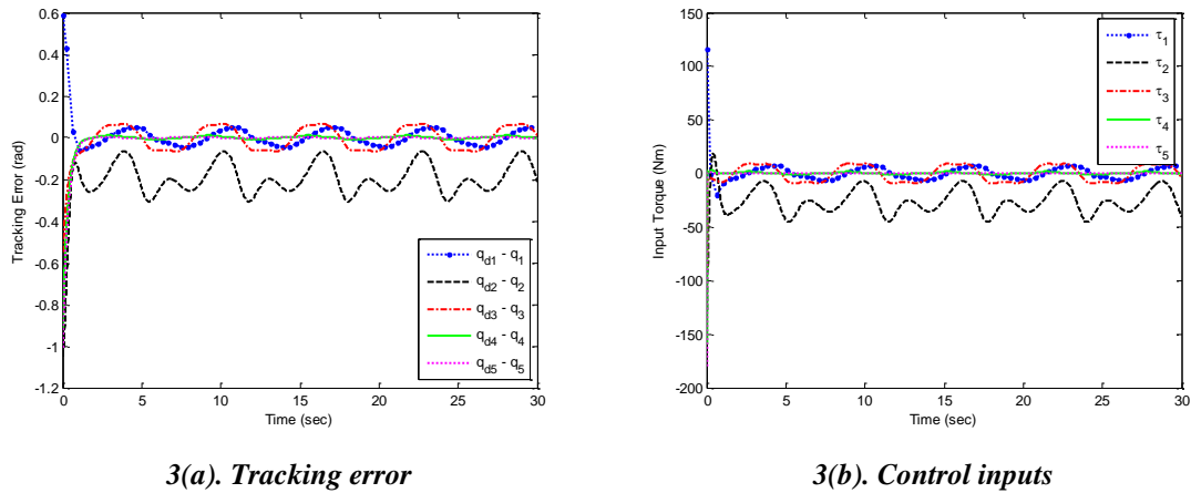
Figure 3. The results of PD controller
