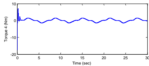
6(k). Control input to joint 4
