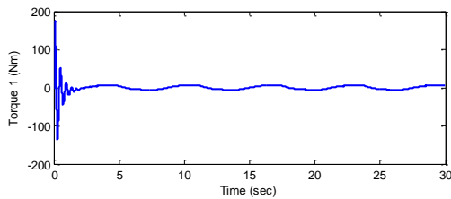
6(h). Control input to joint 1
