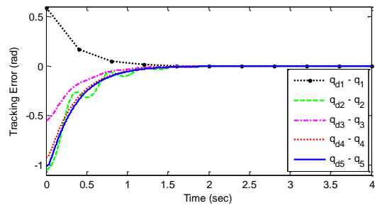
6(g). closer view of the tracking error between 0 and 4 seconds
