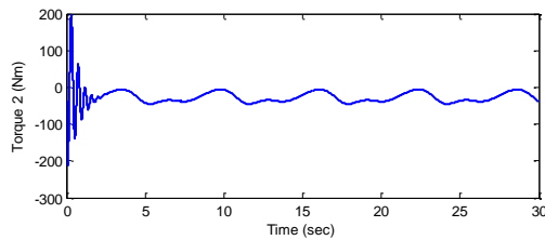
6(i). Control input to joint 2
