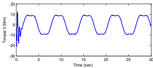
6(j). Control input to joint 3
