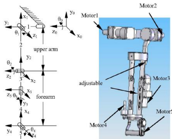
Figure 1. The model of 5-DOF upper-limb exoskeleton robot
