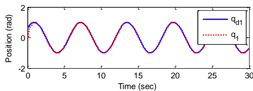
6(a). The position tracking of q_1 to the desired trajectory q_{d1}
