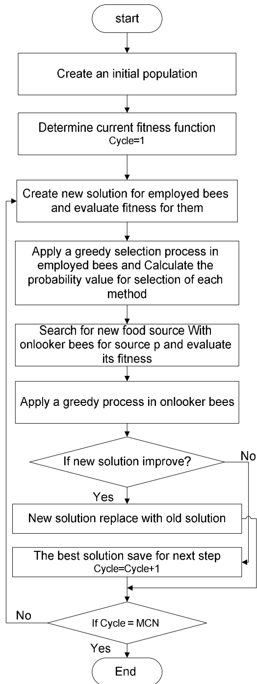
Figure1. Implementation of bee algorithm
